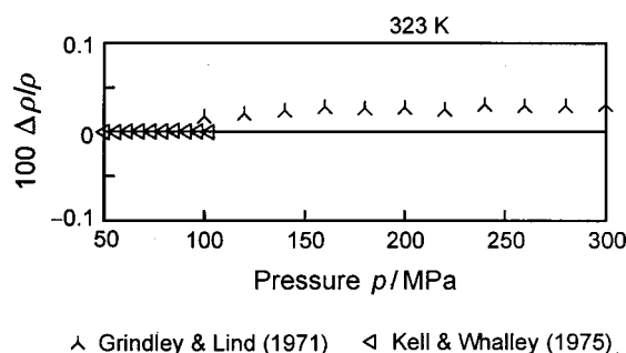
FIG. 4.2. Percentage density deviations 100\Delta\rho/\rho = 100(\rho_{\text{exp}} - \rho_{\text{calc}})/\rho_{\text{exp}} of experimental p\rho T data of Grindley and Lind (1971) and Kell and Whalley (1975) from values calculated from a preliminary equation of state.
