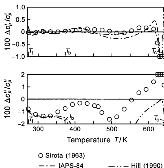
FIG. 7.7. Percentage deviations of the experimental data of the isobaric heat capacity of the saturated liquid c'_p and the isobaric heat capacity of the saturated vapor c''_p from the corresponding values calculated from IAPWS-95, Eq. (6.4). Values calculated from IAPS-84 and the equation of Hill (1990) are plotted for comparison: 100\Delta c'_p/c'_p = 100(c'_{p,\text{exp}} - c'_{p,\text{calc}})/c'_{p,\text{exp}} , 100\Delta c''_p/c''_p = 100(c''_{p,\text{exp}} - c''_{p,\text{calc}})/c''_{p,\text{exp}} .
