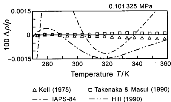
FIG. 7.13. Percentage density deviations 100\Delta\rho/\rho=100(\rho_{\text{exp}}-\rho_{\text{calc}})/\rho_{\text{exp}} between highly accurate experimental p\rho T data along the isobar p=0.101325\text{ MPa} and values calculated from IAPWS-95, Eq. (6.4). Values calculated from IAPWS-84 and the equation of Hill (1990) are plotted for comparison.
