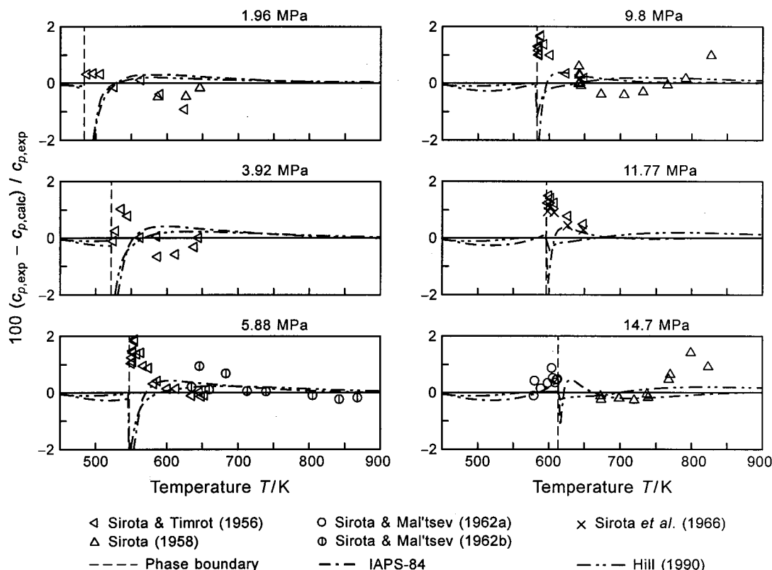
FIG. 7.32. Percentage deviations between experimental data of the isobaric heat capacity c_p and values calculated from IAPWS-95, Eq. (6.4). Values calculated from IAPS-84 and the equation of Hill (1990) are plotted for comparison.
